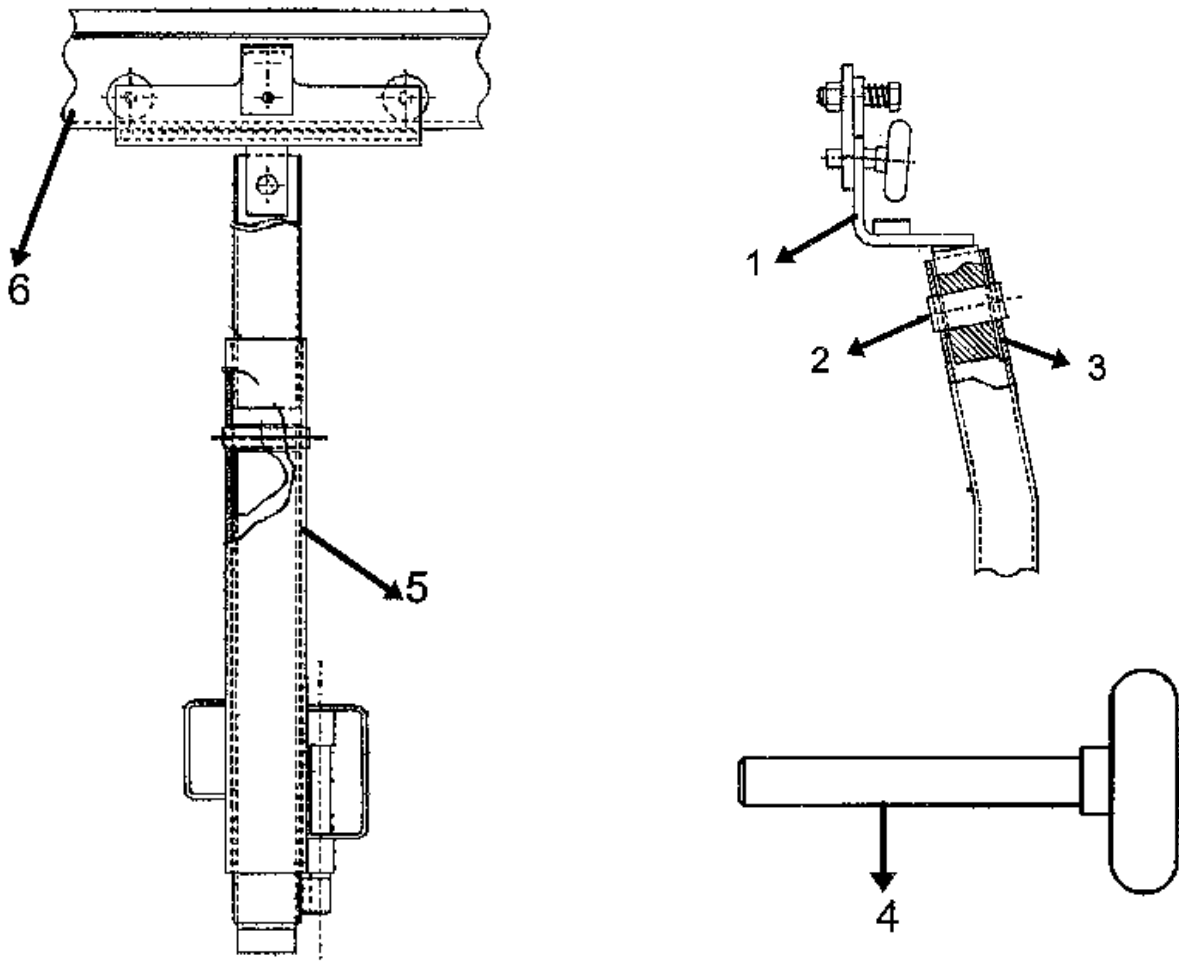
FRT-224-01011 - SLIDE POST ASSEMBLY – SUIT 2770mm HIGH APERTURE
