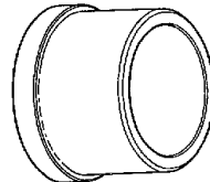
SXT-02-2069 ROCKWELL DRIVE 38mm I.D x 48mm O.D 39mm LONG STEEL
