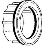
SXT-02-2051 INNER BUSH WHITE 38mm I.D x 48mm O.D NYLON
