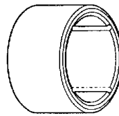
SXT-03-3007 ROCKWELL DRIVE-PINK 38mm I.D x 48mm O.D 30mm LONG NYLON
